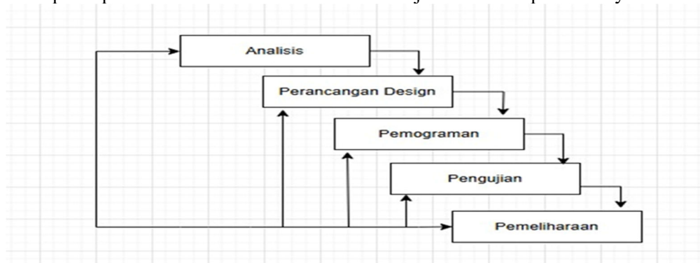
Gambar 1. Metode Waterfall
