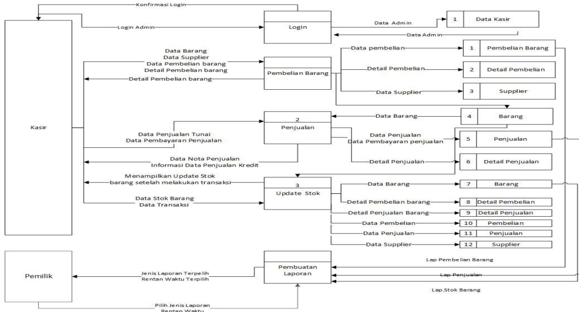
Gambar 3. DFD Level 1
