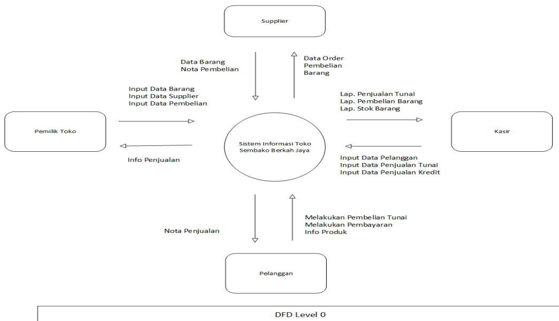
Gambar 2. DFD Level 0
