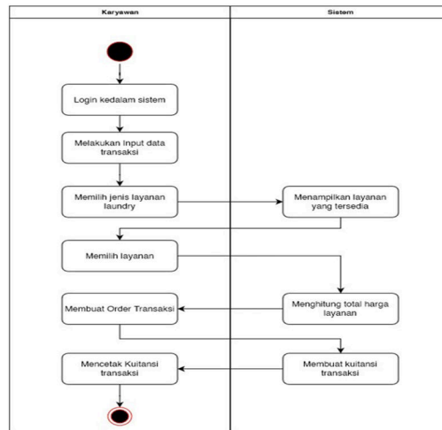
Gambar 2. Activity Diagram
