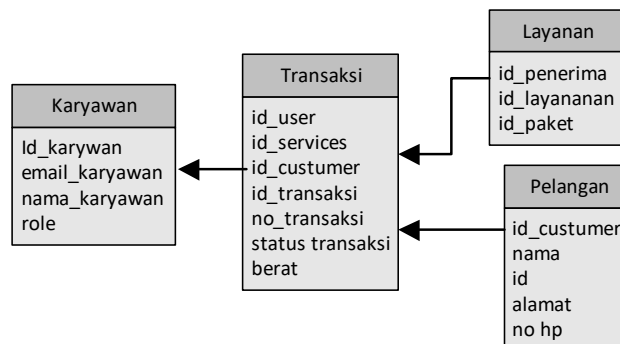
Gambar 3. Class Diagram
