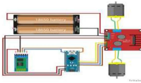
Figure 14. Wireless Control Electronic Hardware System Design
