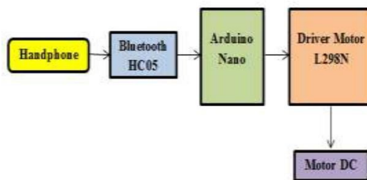
Figure 13. Block Diagram of Rice Plow Tool Control
