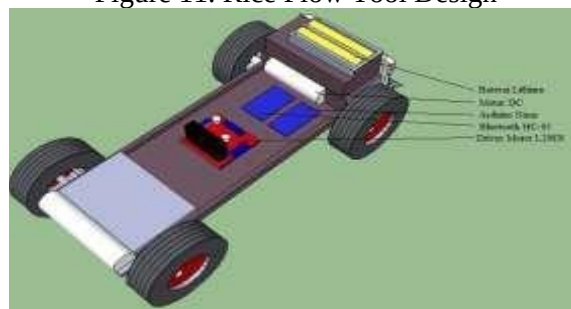
Figure 12. Mechanical Components of the Rice Plow Equipment System
