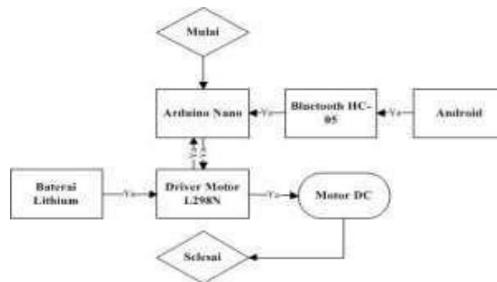
Figure 15. Program Flowchart
