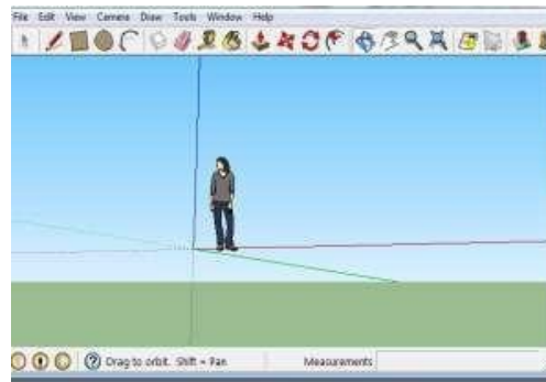
Figure 8. Google SketchUp 8
