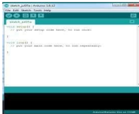
Figure 6. Arduino IDE
