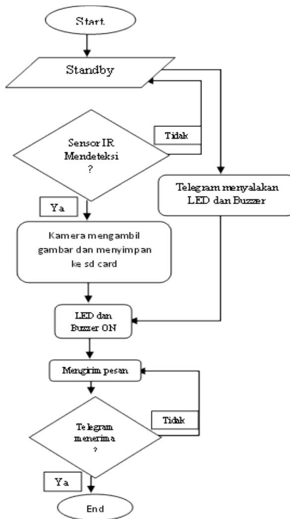
Figure 1. Program Flowchart
